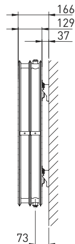
3P/30, profile
